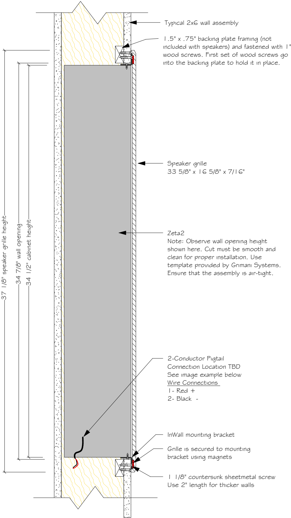
Zeta2 - In-Wall Mounting Detail
