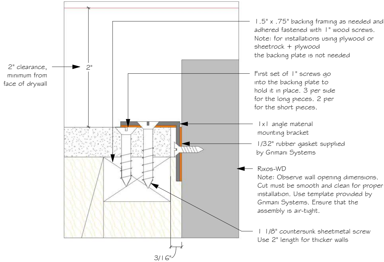
Rixos-WD - In-Wall Proud Mounting Detail
