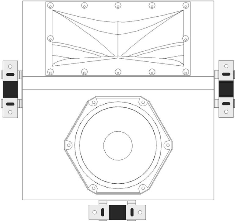
On-Ceiling See sheet A14.5 for installation details
