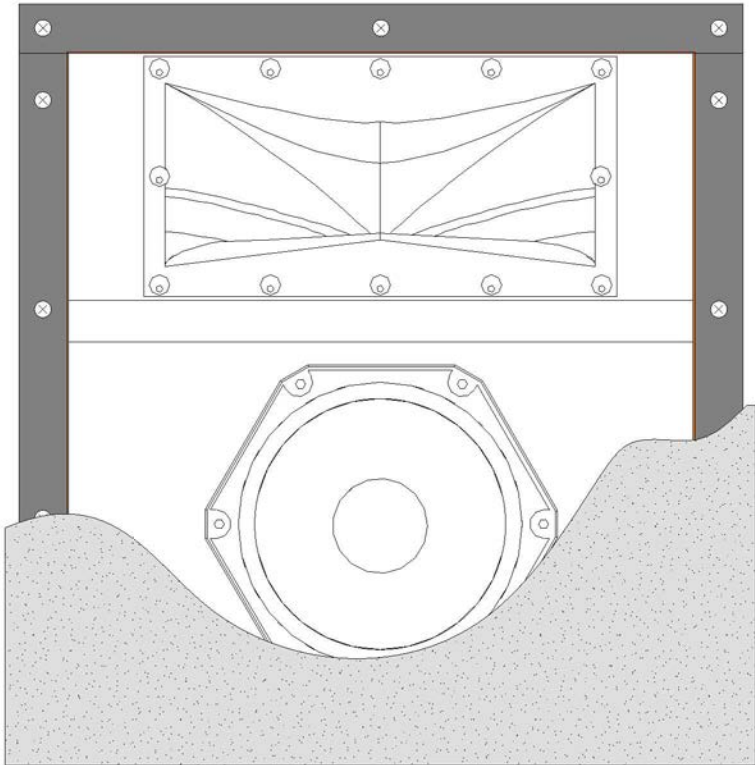
In-Ceiling See sheet A14.2 and A14.3 for installation details
