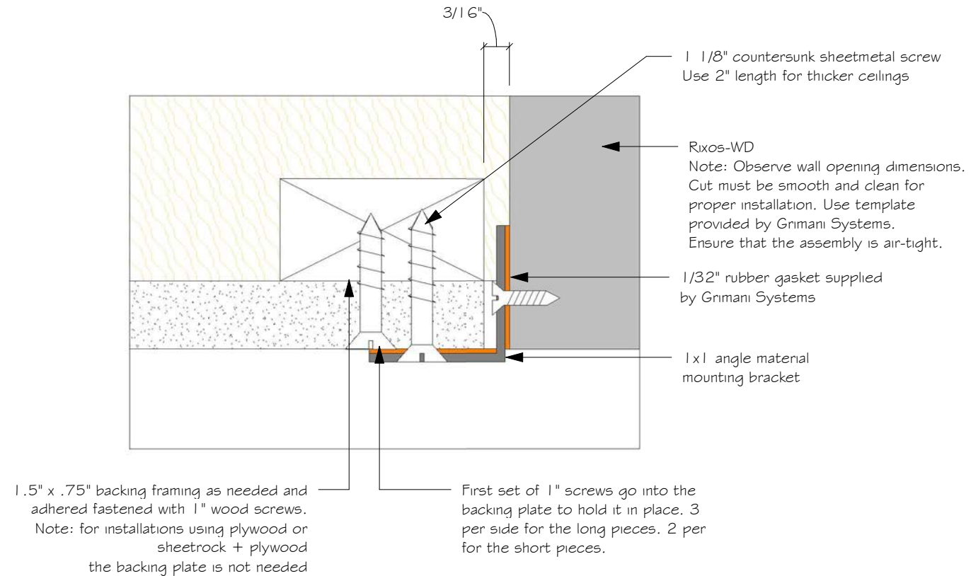
Rixos-WD - In-Ceiling Proud Mounting Detail
