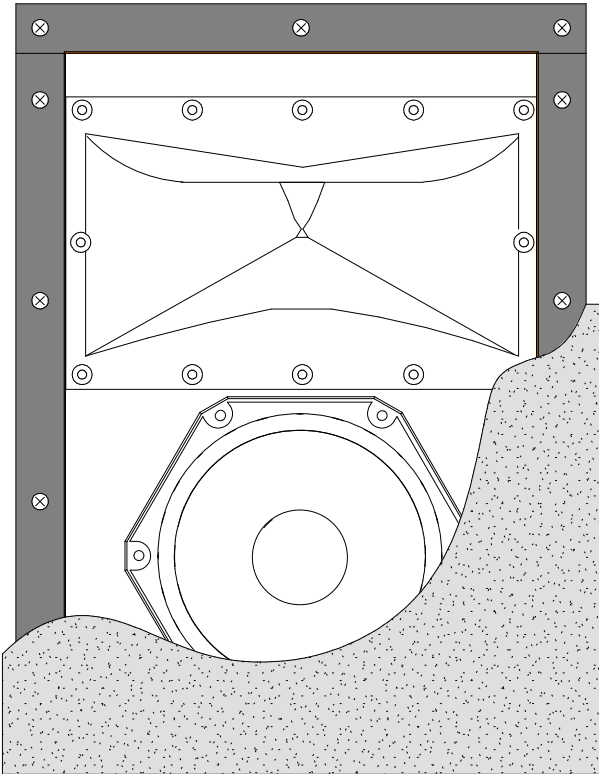
In-Wall See sheet A 9.2 and A 9.3 for installation details
