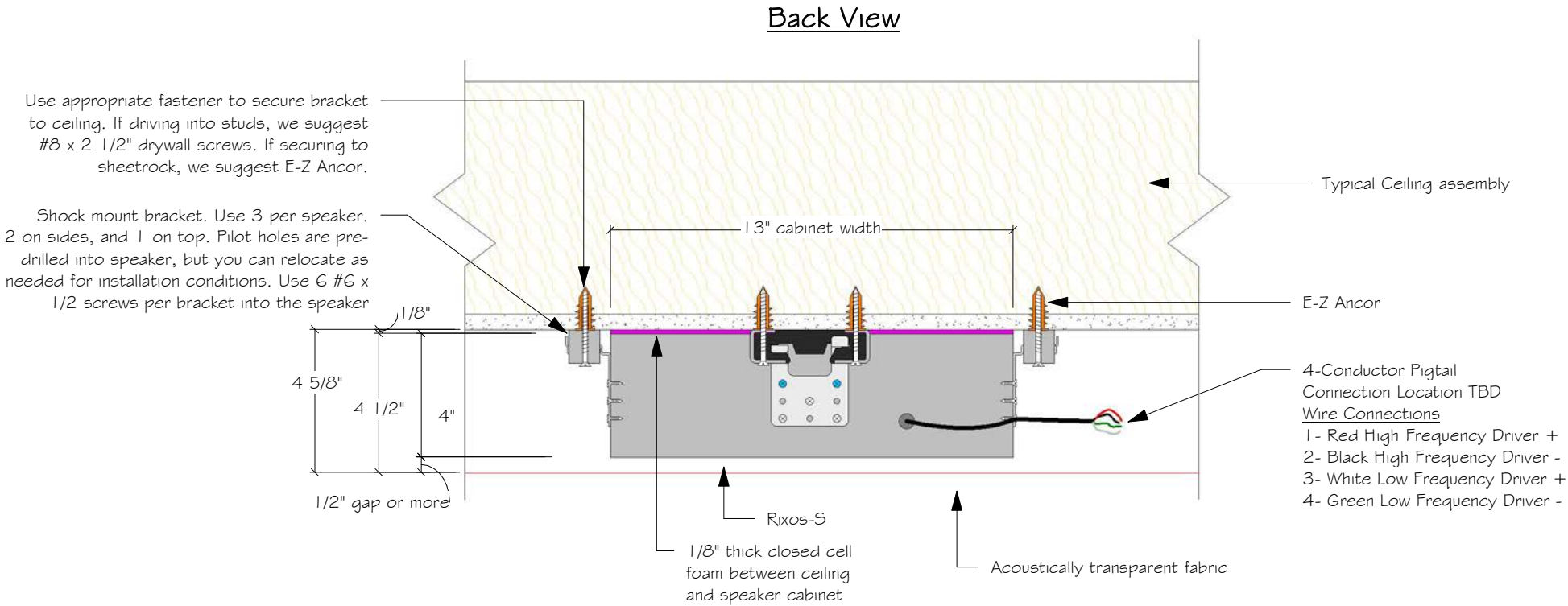
Rixos-S - On-Ceiling Mounting Detail
