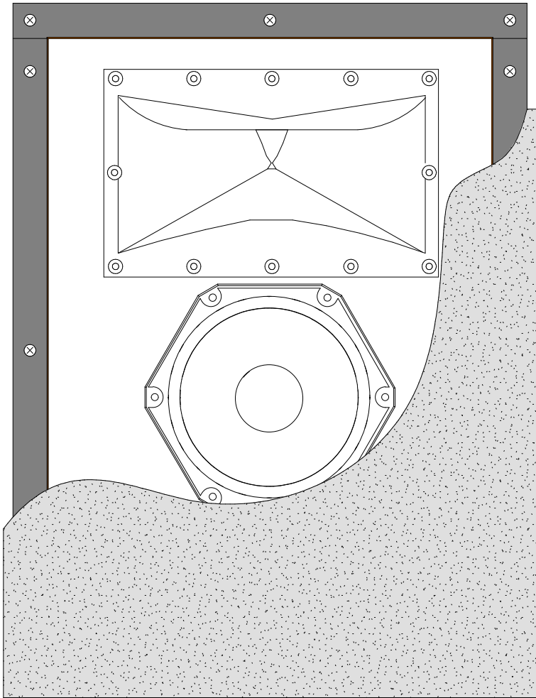
Bezel or Flush Mount Grille, Right Angle Metal Flanges
