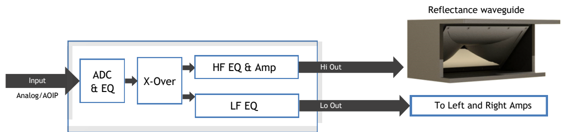
EQ/Amp/Spkr Block Diagram
